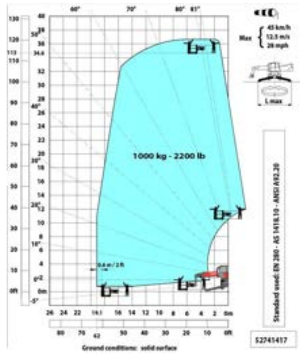
Machine on lowered stabilisers with 1000 kg platform Metric
